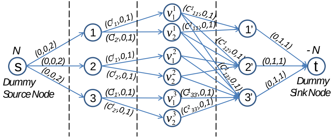
Figure 2. An example of Problem P minimum cost flow network with two vessel types ( K=2 ) and three ports ( N=3 ).
