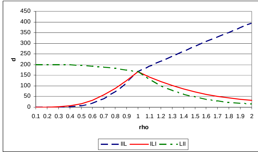
Figure 3. Maximum unit processing time for a lot machine under item-machine dominance
