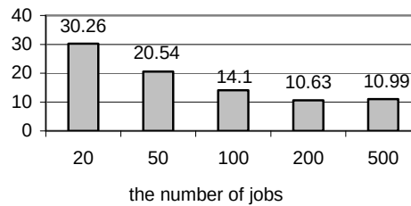
Fig. 1. The criterion value improvement with regard to the initial solution for different sizes of input instances
