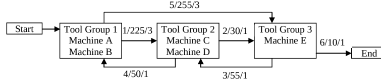
Figure 2. The mini-fab model [2]
